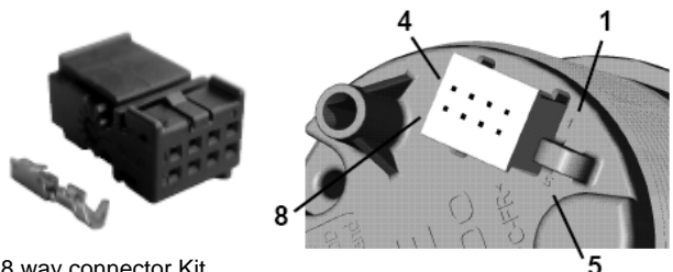
8 way connector Kit p/n A2C59510850
