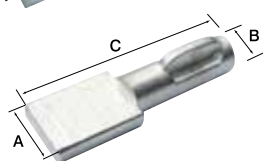
Drive key 230.064
